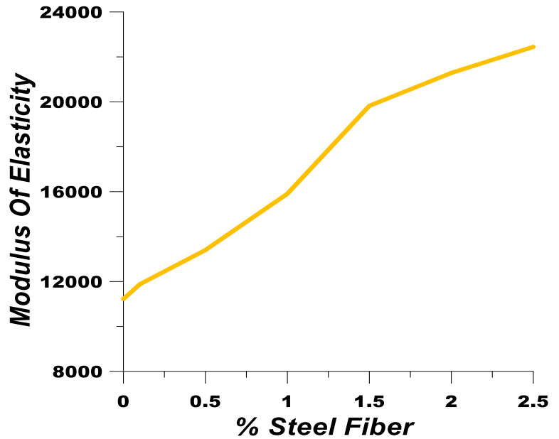
Fig. 7 Modulus Of Elasticity Test
