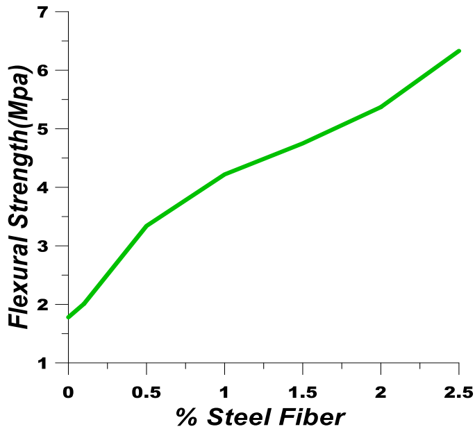
Fig. 6 Flexural Strength Test
