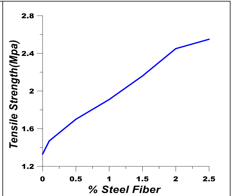
Fig. 9 Tensile Strength Test
