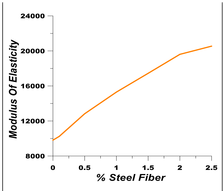
Fig. 11 Modulus Of Elasticity Test
