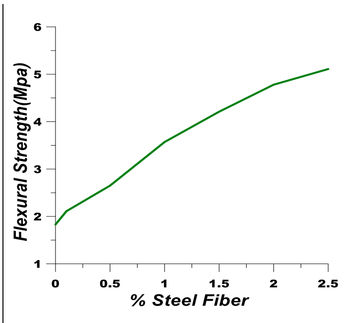
Fig. 10 Flexural Strength Test
