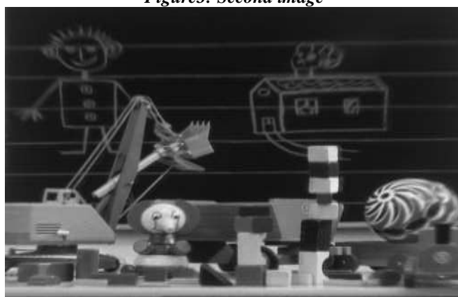
Figure4: Original image
