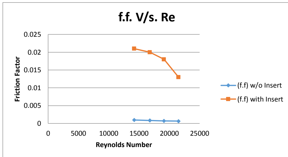
Fig 6: Friction factor vs. Reynolds Number
