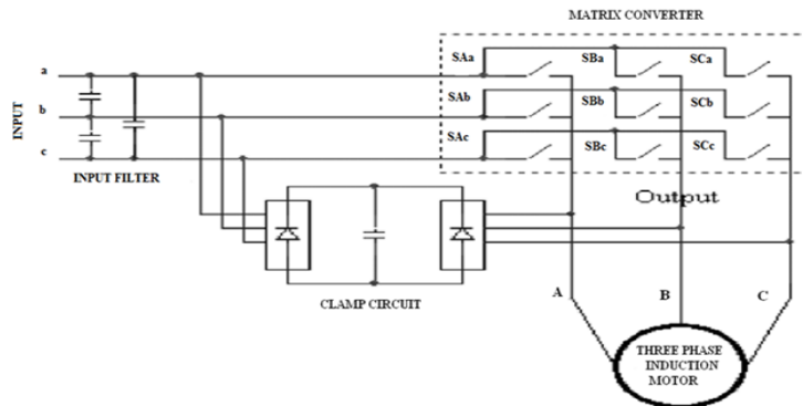
Fig.2 The practical scheme of matrix converter drive
