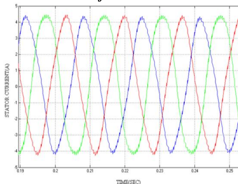
Stator Current on No Load Waveform For Venturini Modulation Technique
