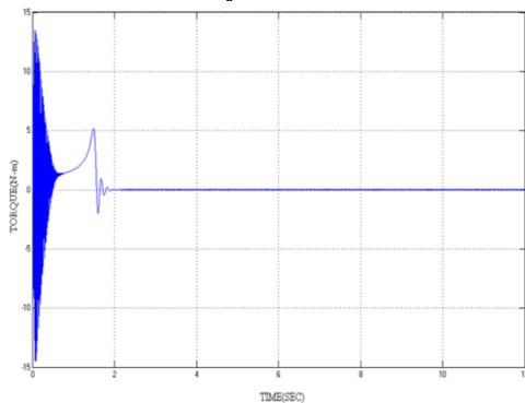
Torque Response on No Load Waveform For Venturini Modulation Technique
