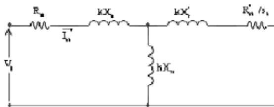
Fig.1.K th harmonic equivalent circuit of induction motor
