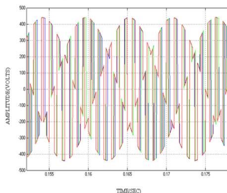
Output Voltage Waveform For Venturini Modulation Technique
