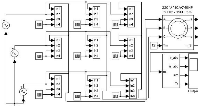
Fig.4 Block diagram of matrix converter fed Induction motor drive
