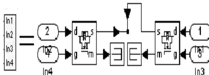
Fig.5 Subsystem of bi-directional switch
