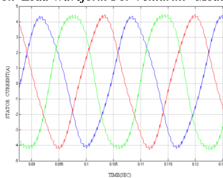
Rotor Current on Load Waveform For Venturini Modulation Technique
