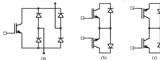
Fig.3 Bi-directional switch topologies using unidirectional switches:
