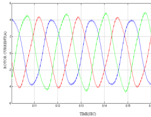
Speed Response on Load Waveform For Venturini Modulation Technique
